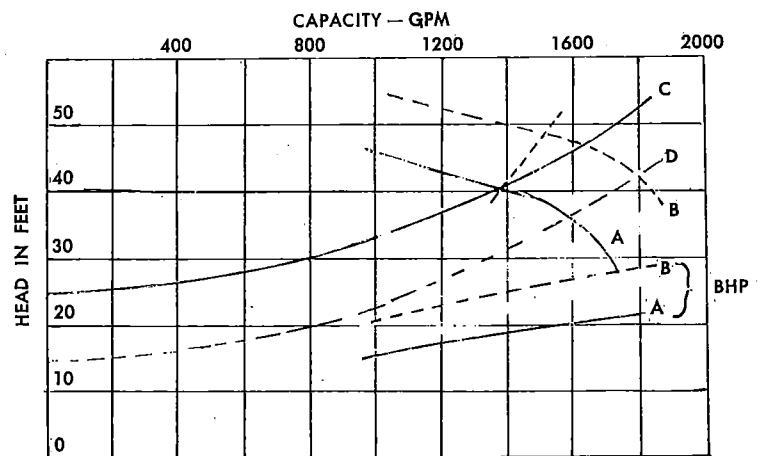
A—Basic Pump Characteristic Curve B—Calculated Affinity Curve C—Basic System Curve D—Auxiliary System Curve
