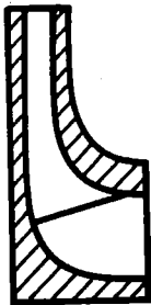
Fig. 2. Single suction, horizontal or vertical centrifugal pumps with narrow port impellers have low capacities and deliver high heads. Specific speed range is 500 to 1000.
